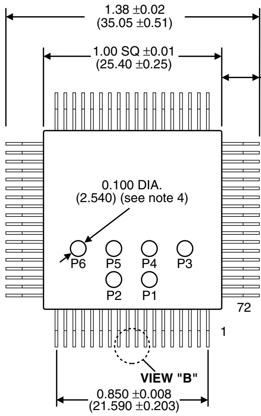
BOTTOM VIEW
